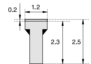
Izgara Kesiti Grating Section
