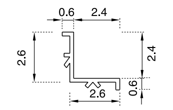
Izgara Profil Grating Profile
