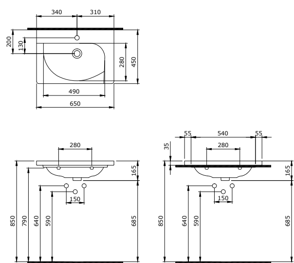
1009-001-0126 Taormina Arch Etajerli Lavabo 65 cm Taormina Arch Vanity Basin 65 cm Taormina Arch Lavabo da Incasso 65 cm
